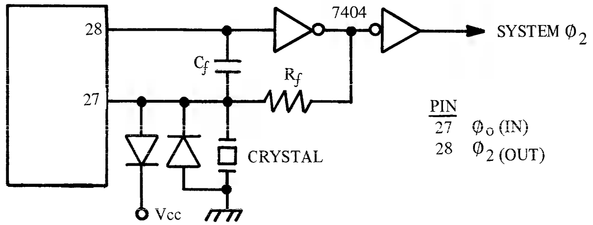
MCS6503,4,5 Parallel Mode Crystal Controlled Oscillator
